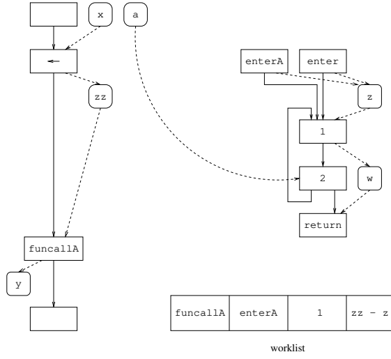
Figure 2: Instruction graph after initialization.
